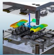
Plastic Injection
