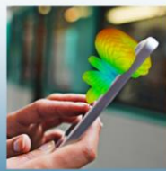
Electromagnetics
